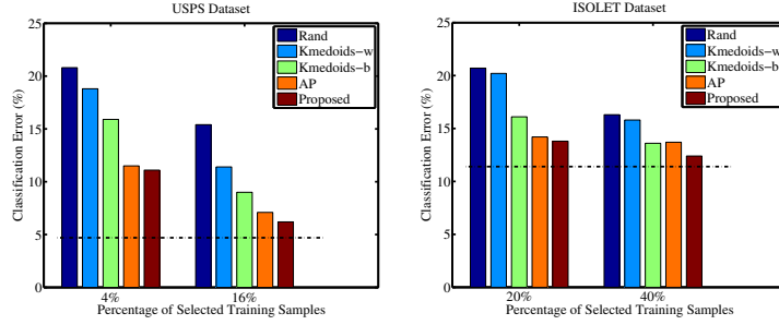
Figure 6: Classification error on the USPS (left) and ISOLET (right) datasets using representatives obtained by different algorithms. Horizontal axis shows the percentage of the selected representatives from each class (averaged over all classes). Dashed line shows the classification error (%) using all the training samples.
